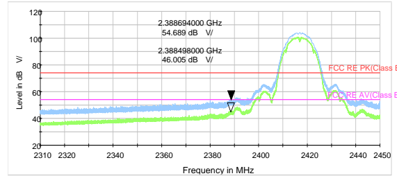
802.11b-Channel 2 Peak & Average
