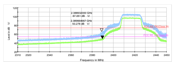
802.11n HT20 -Channel 2 Peak & Average
