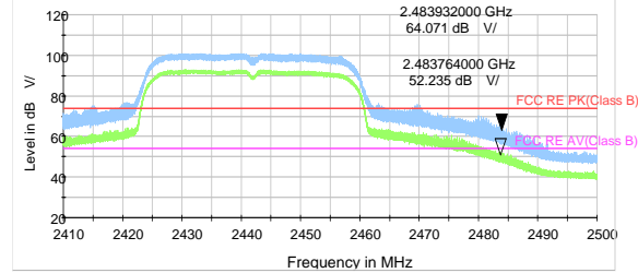
802.11n HT40 -Channel 7 Peak & Average
