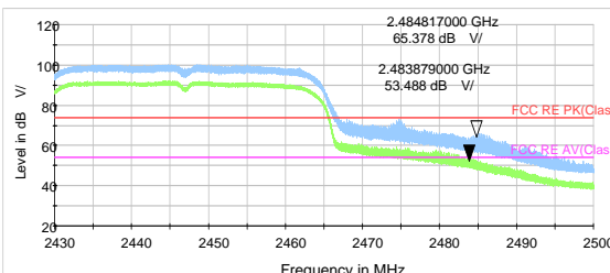
802.11n HT40 -Channel 8 Peak & Average
