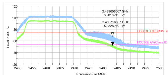
802.11g-Channel 11 Peak & Average
