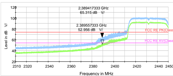
802.11n HT40 -Channel 5 Peak & Average
