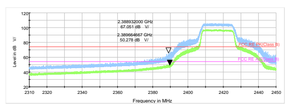
802.11n HT20 -Channel 2 Peak & Average
