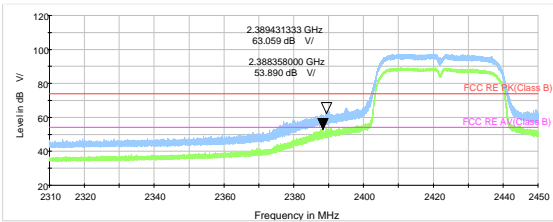
802.11n HT40 -Channel 3 Peak & Average
