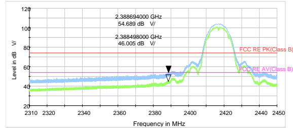
802.11b-Channel 2 Peak & Average
