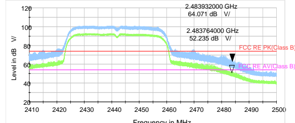
802.11n HT40 -Channel 7 Peak & Average
