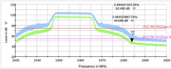
802.11n HT20 -Channel 10 Peak & Average
