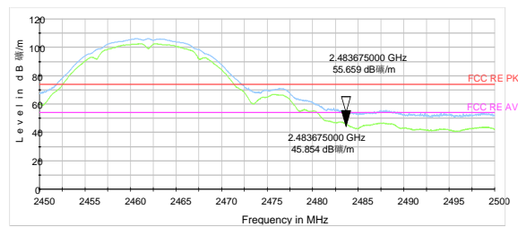
802.11b-Channel 11 Peak & Average
