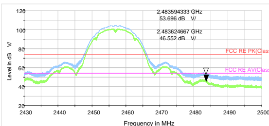
802.11b-Channel 10 Peak & Average
