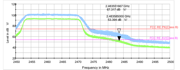
802.11n HT20 -Channel 11 Peak & Average
