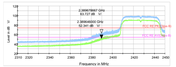
802.11n HT40 -Channel 4 Peak & Average
