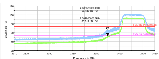
802.11n HT20 -Channel 1 Peak & Average
