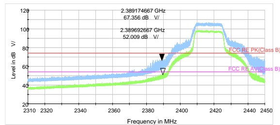
802.11g-Channel 2 Peak & Average
