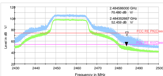
802.11g-Channel 10 Peak & Average
